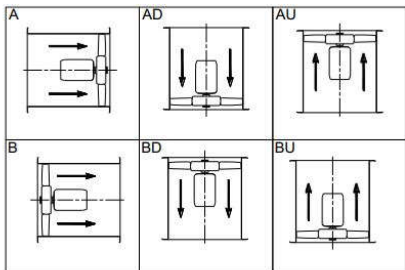
Fig. 2-2 Flow indications
