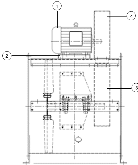
Fig. 5-5 Assembly of version 9 axial fans
