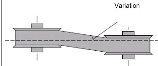
Fig. 9.3 Parallel misalignment
