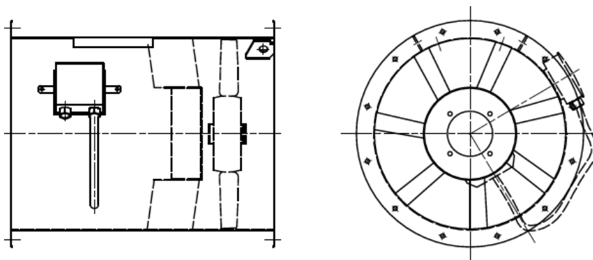
Fig. 5-8 Example of positioning of external terminal box
