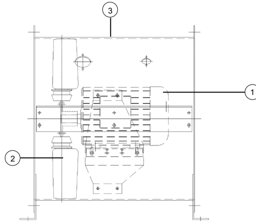
Fig. 5-3 Assembly of version 4 axial fans
